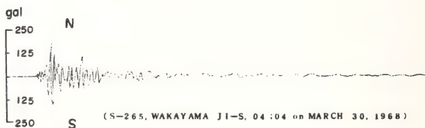
Fig. 15 Accelerograms recorded at Wakayama port
